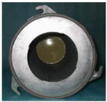
ALU TOP 3L Sizes: 145, 218, 325 Note: Fixing centre line: 145= 203mm, 218= 263mm, 325= 394 mm Freudenberg's LP 145= 180mm
